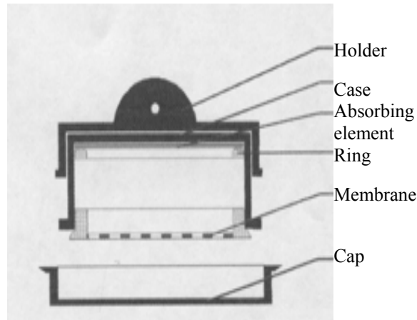
Fig. 1. Passive sampler for determination of nitrogen dioxide concentration
