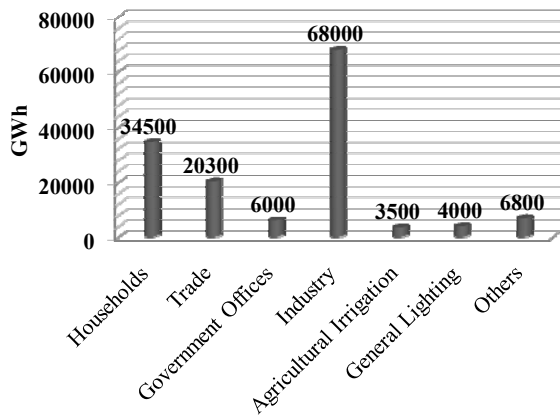
Fig. 1. Distribution of electrical energy used in Turkey. Based on EIE 2008
