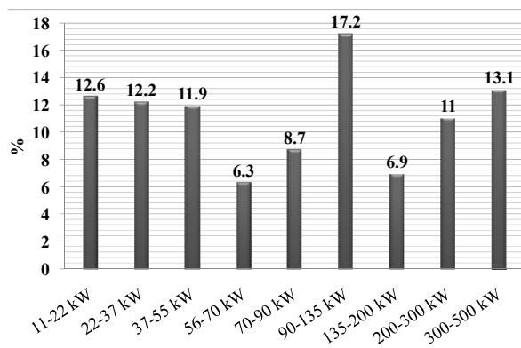
Fig.3. Power distribution among electric motors used in industry. Based on EIE 2008
