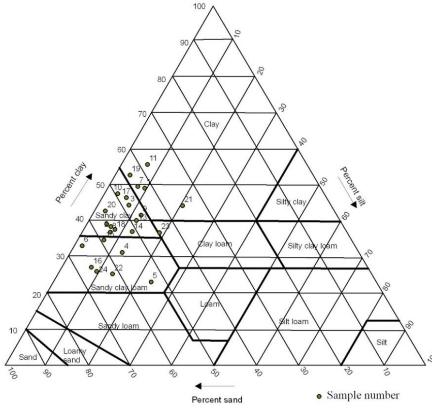
Fig. 1B. Textural Classes –the Kallada (Upper layer)
