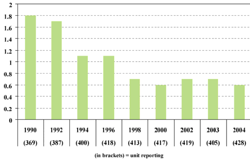
Fig. 13. Unplanned scrams per 7000 hours critical (IAEA, 2006)
