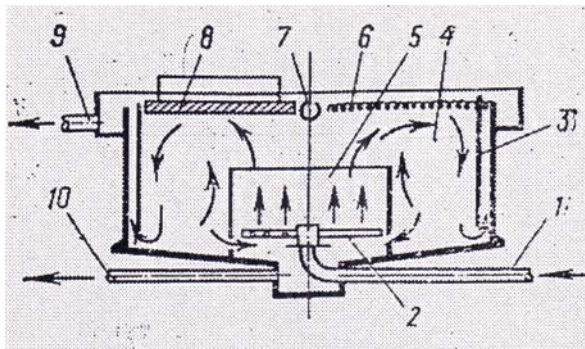
Fig. 4. Typical flotator of Soyuzvodokanalproyekt: 1 – water delivery with reagent and air-water mixture; 2 – distribution device (Segner-wheel); 3 – semisubmerged partition; 4 – flotation zone; 5 – ring-shaped partition; 6 – foam; 7 – radial foam-collecting tray; 8 – scraper; 9 – purified water outlet; 10 – washout and sediment withdrawal pipeline
