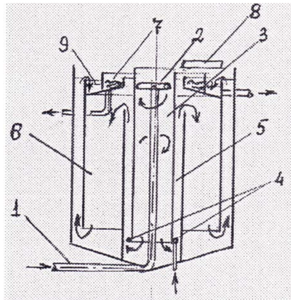
Fig. 7. Pressure flotator, “Stroyengineering SM” L.L.C. 1 – water-reagent mixture feed pipeline; 2 – distribution device; 3 – flocc formation chamber; 4 – ring-shaped perforated pipeline for delivery of air-water mixture from saturator; 5 – mixing chamber; 6 – flotation chamber; 7 – foam-collecting tray; 8 – scraper; 9 – purified water intake tray.
