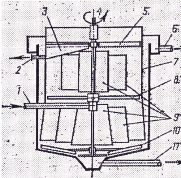
Fig. 6. VNI VODGEO flotator. 1 – waste water and air-water mixture feed pipeline; 2 – foam products outlet pipeline; 3 – foam-collecting tray; 4 – drive; 5 – scraper; 6 – purified water outlet pipeline; 7 – semisubmerged partition; 8 – rotating distribution device; 9 – coaxial partitions; 10 – slurry scraper; 11 – slurry pipeline
