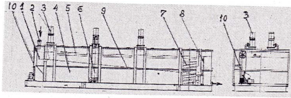
Fig. 8. Impeller flotator, "Stroyengineering SM" L.L.C. 1 – intake chamber; 2 – waste water inlet; 3 – disperser drive; 4 – flotator housing; 5 – foam intake windows; 6 – impeller disperser; 7 – thin-layer unit; 8 – overflow; 9 – foam intake tray; 10 – foam-removing scraper drive
