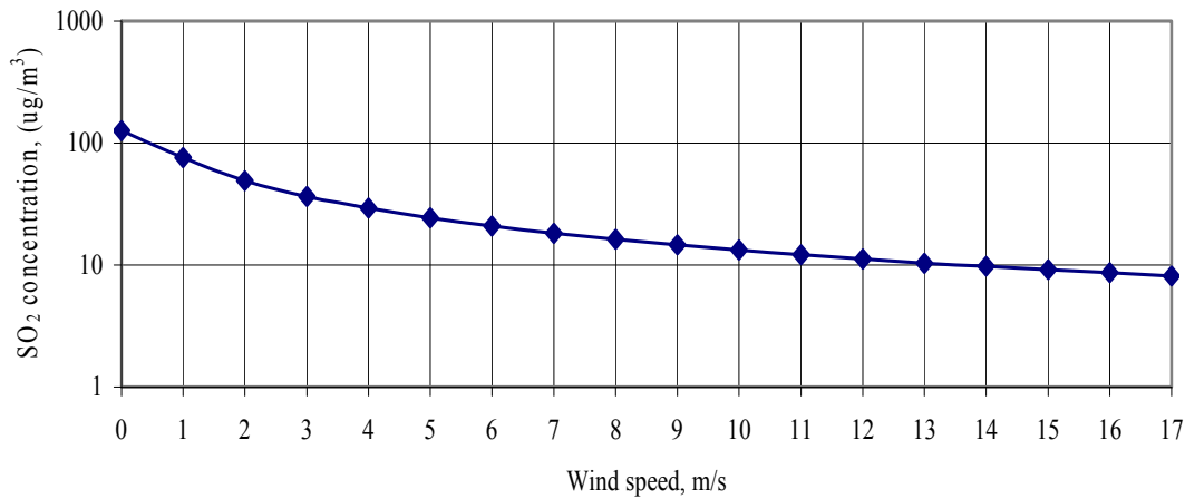
Fig. 7. SO 2 concentration in a monitoring station in accordance with CALPUFF, when one-way but different speed winds (μg/m) are blowing
